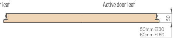
Active door leaf
