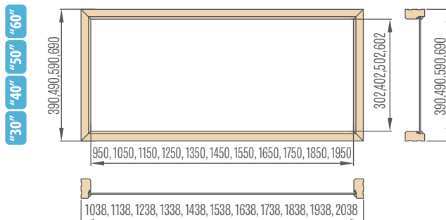
Top lights for fixed door frame in double doors
