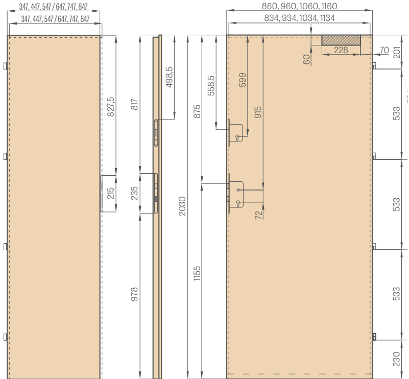
Side panel / inactive door leaf
